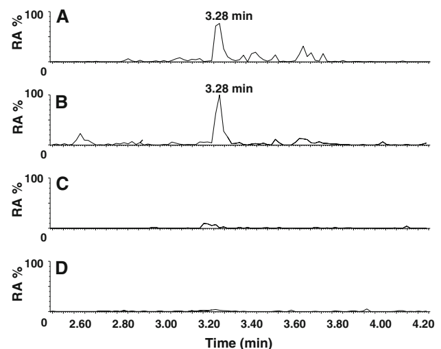
Fig. 2 Location of modified peptide ^{170}\text{VK}^{176}_{\text{CML}}\text{R}^{183} Extracted ion chromatograms at a m/z 826 (2 + charge state) and b m/z 551 (3 + charge state) for \beta CN incubated with glucose for 4 h show one major peak at 3.28 min. Extracted ion chromatograms at c m/z 826 and d m/z 551 for native \beta CN show no peak at 3.28 min. The chromatograms are normalised to the same scale
